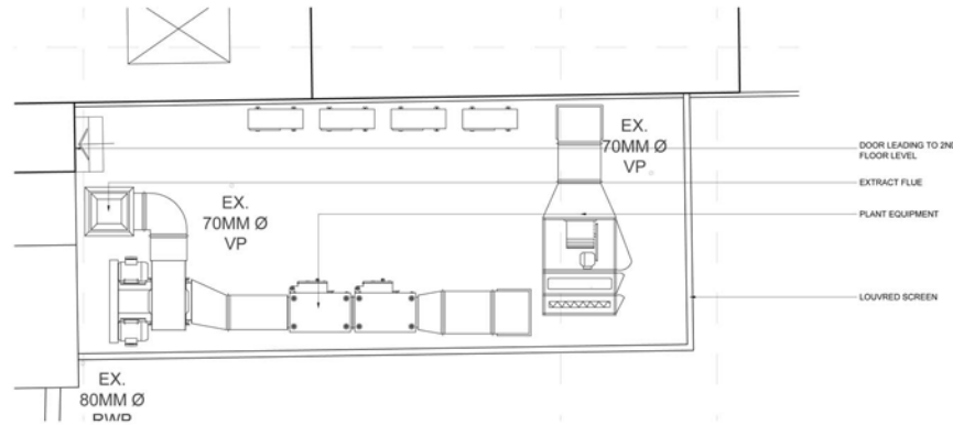
03 PLANT DECK PLAN 1:50 @ A1
