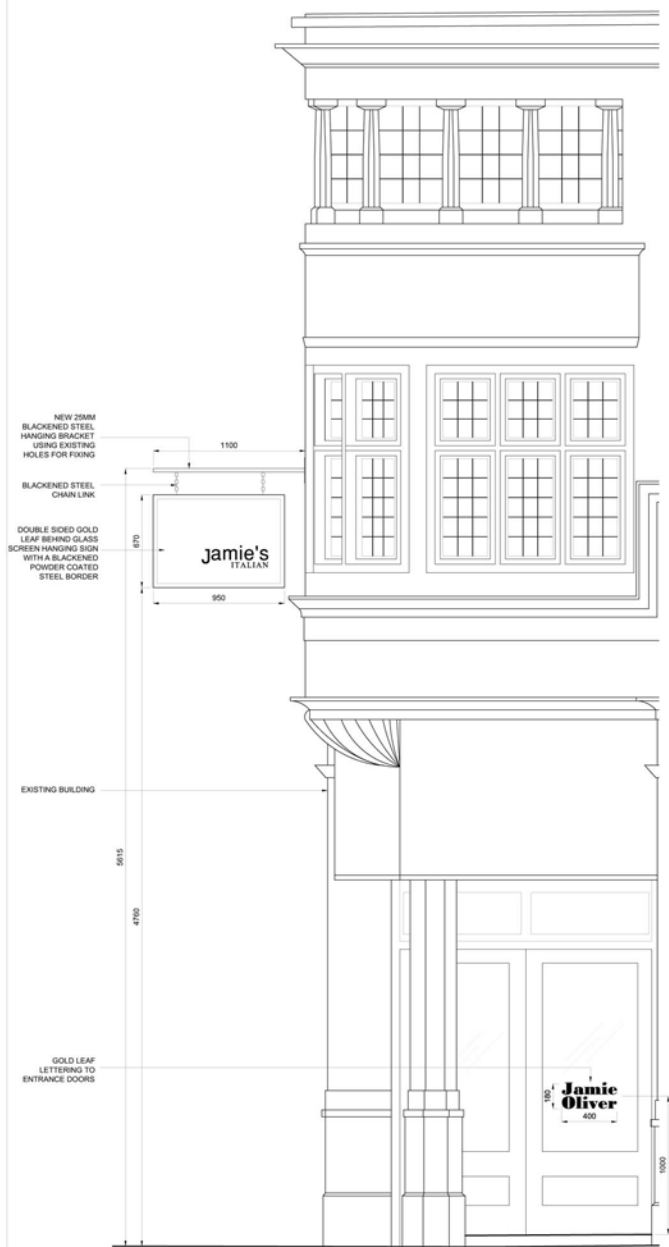
01 HANGING SIGN - NORTH ELEVATION 1:20 @ A1
