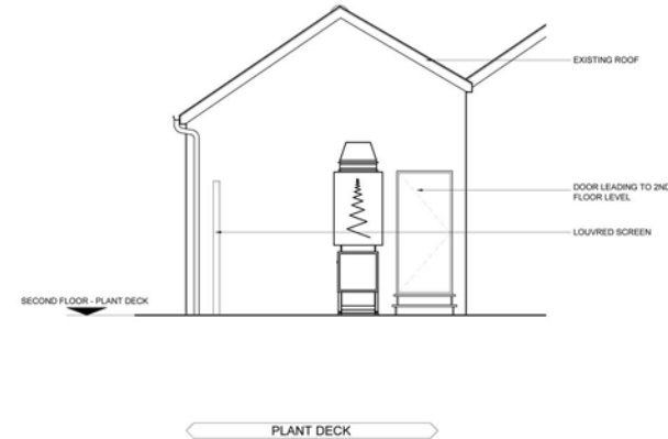
02 PLANT DECK ELEVATION B 1:50 @ A1
