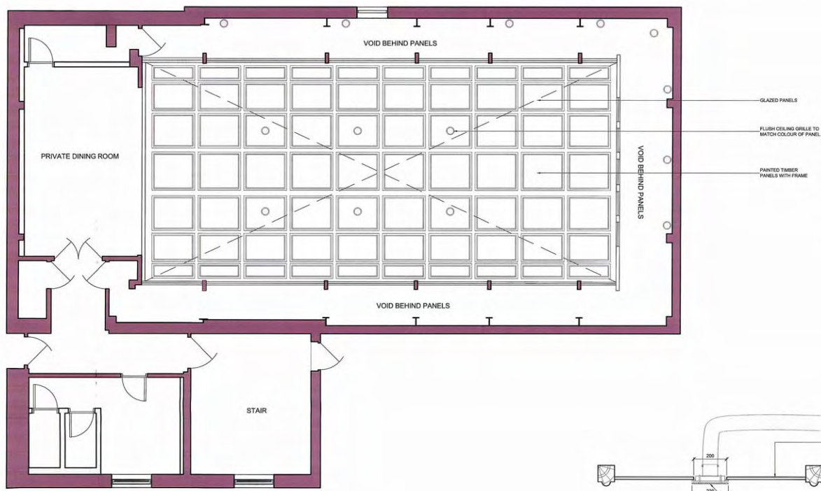
01 SECOND FLOOR ROOF PLAN 1:50 @ A1
