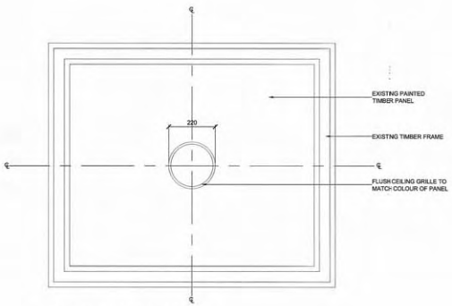
04 PLAN OF ROOF PANEL 1:10 @ A1
