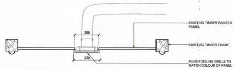
03 SECTION OF ROOF PANEL 1:10 @ A1
