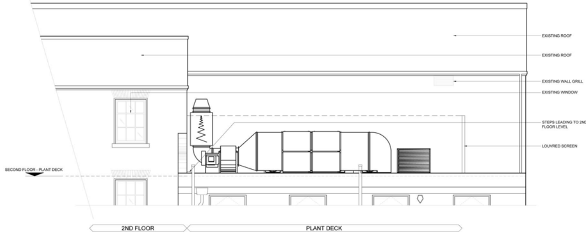
01 PLANT DECK ELEVATION A 1:50 @ A1
