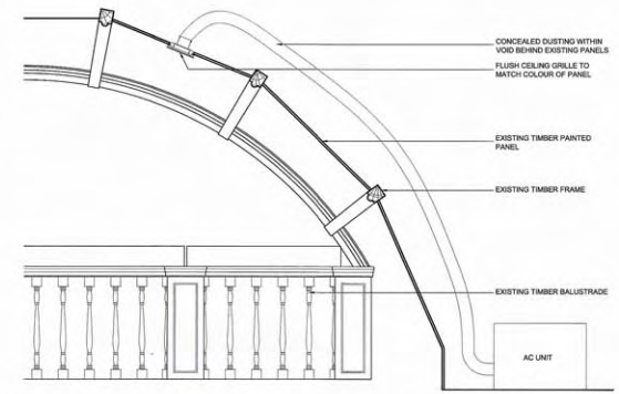
02 SECTION OF ROOF PANELS 1:20 @ A1
