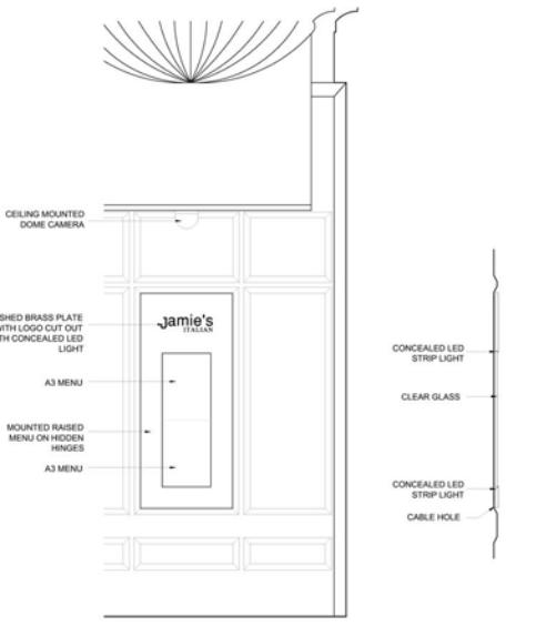
05 MENU BOX ELEVATION 1:10 @ A1
