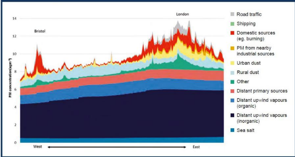
Annual mean PM 2.5 west to east transect across the UK for 2017 from PCM model
