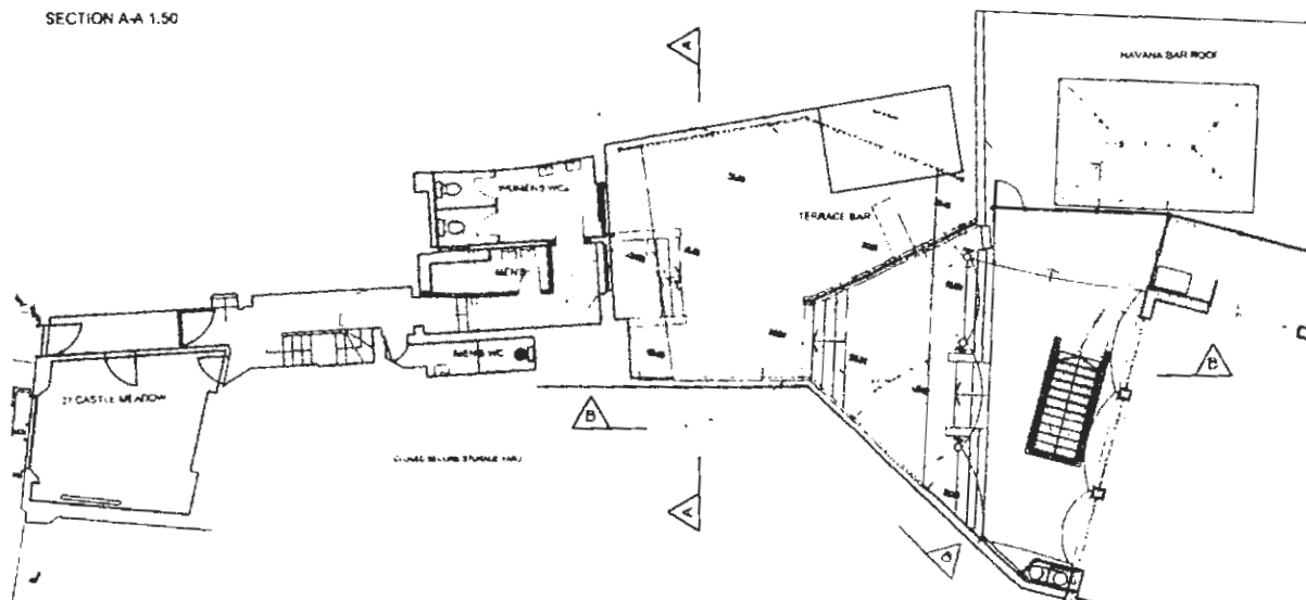
UPPER GROUND LEVEL PLAN 1:50
