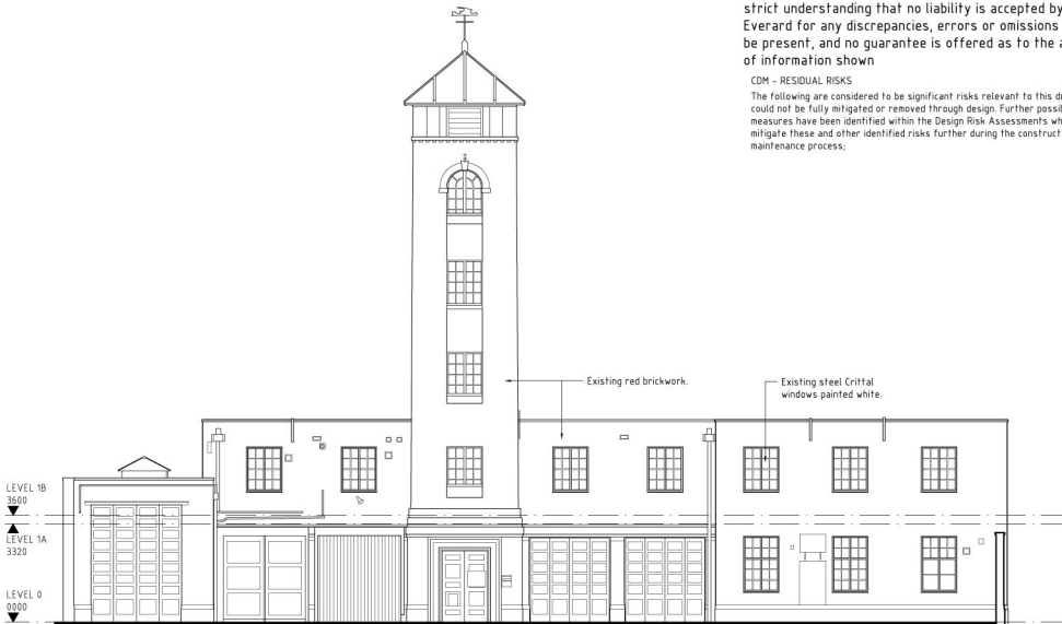
SOUTH COURTYARD ELEVATION
