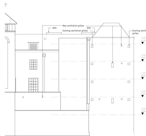
NORTH ELEVATION
