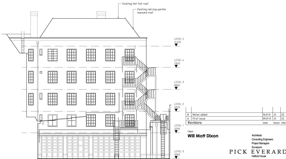
EAST COURTYARD ELEVATION
