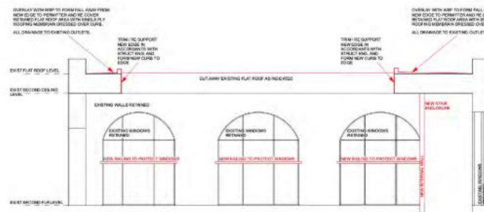
PROPOSED SECTION A-A SCALE 1:100@A1
